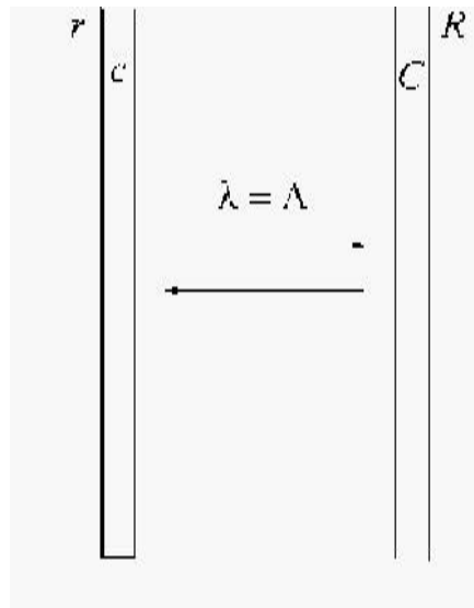
FIG. 1 Setup of Kirchhoff's first proof
