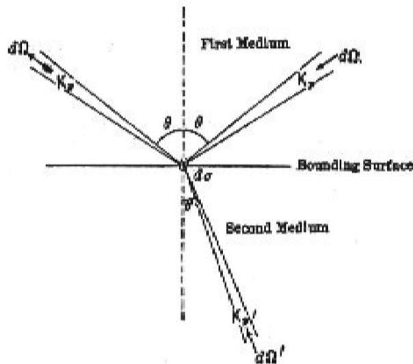
FIG. 4 Planck's diagram of radiation traversing a border between different media. Planck, Theory (ref. 53), 33.
